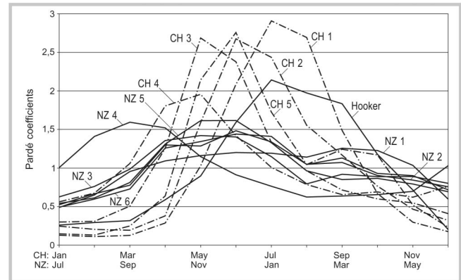
FIGURE 8 River regimes based on Pardé coefficients (monthly mean flows over annual mean flow) for representative catchments of the Swiss (CH) and Southern Alps (NZ), including the Hooker River catchment of the Southern Alps.
