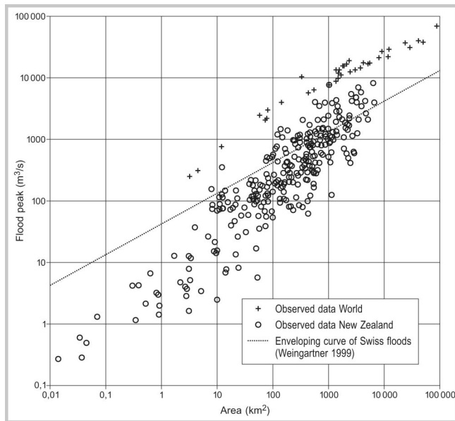
FIGURE 10 Maximum recorded flood peaks from catchments of different drainage area for New Zealand (Pearson 1992) and the world (Costa 1987) compared with the enveloping curve of Switzerland (Weingartner 1999).
